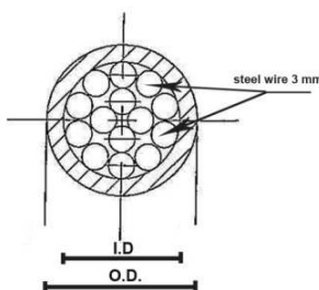
NORMAL THERMAL LANCE
